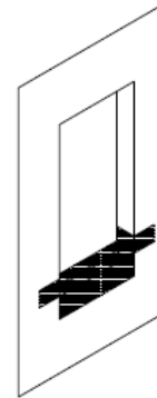
Step 4: Install flexible flashing such as Vycor over plywood backdam and rough opening sill and extend down weather barrier 8" and min 6" up side jamb.
