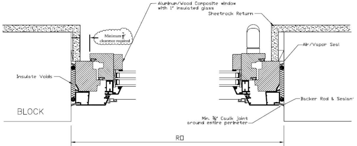
JAMB VIEW
