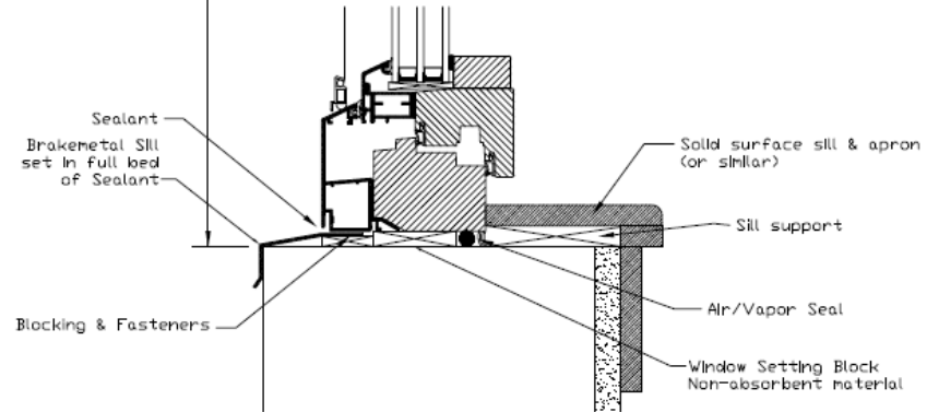
HEAD & SILL VIEW
