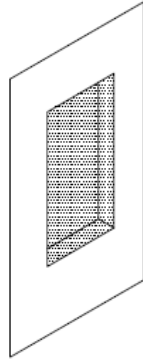
Step 2: Cut out weather barrier that covers rough opening flush with edge of rough opening.
